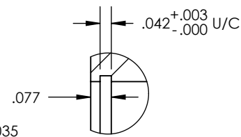
DETAIL C SCALE 2 : 1
