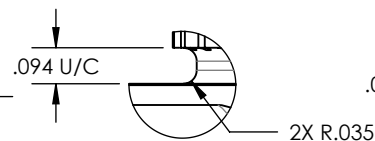
DETAIL B SCALE 2 : 1
